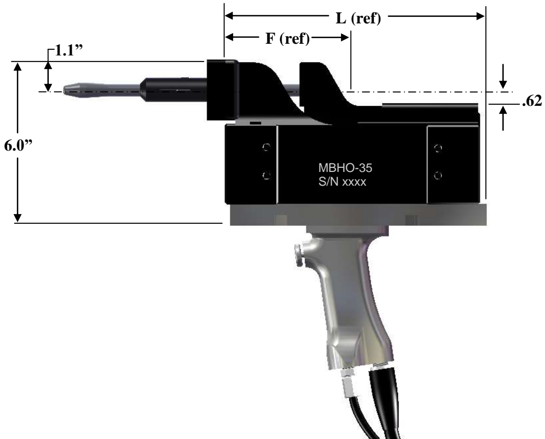
Figure 1.3-2 Medium Brute Hydraulic Offset Measurements
