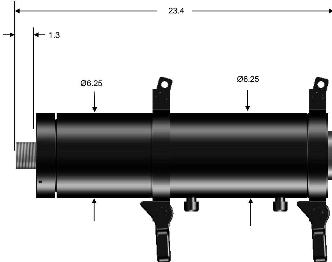
Figure 1.3-2 SB-2A Dimensions
