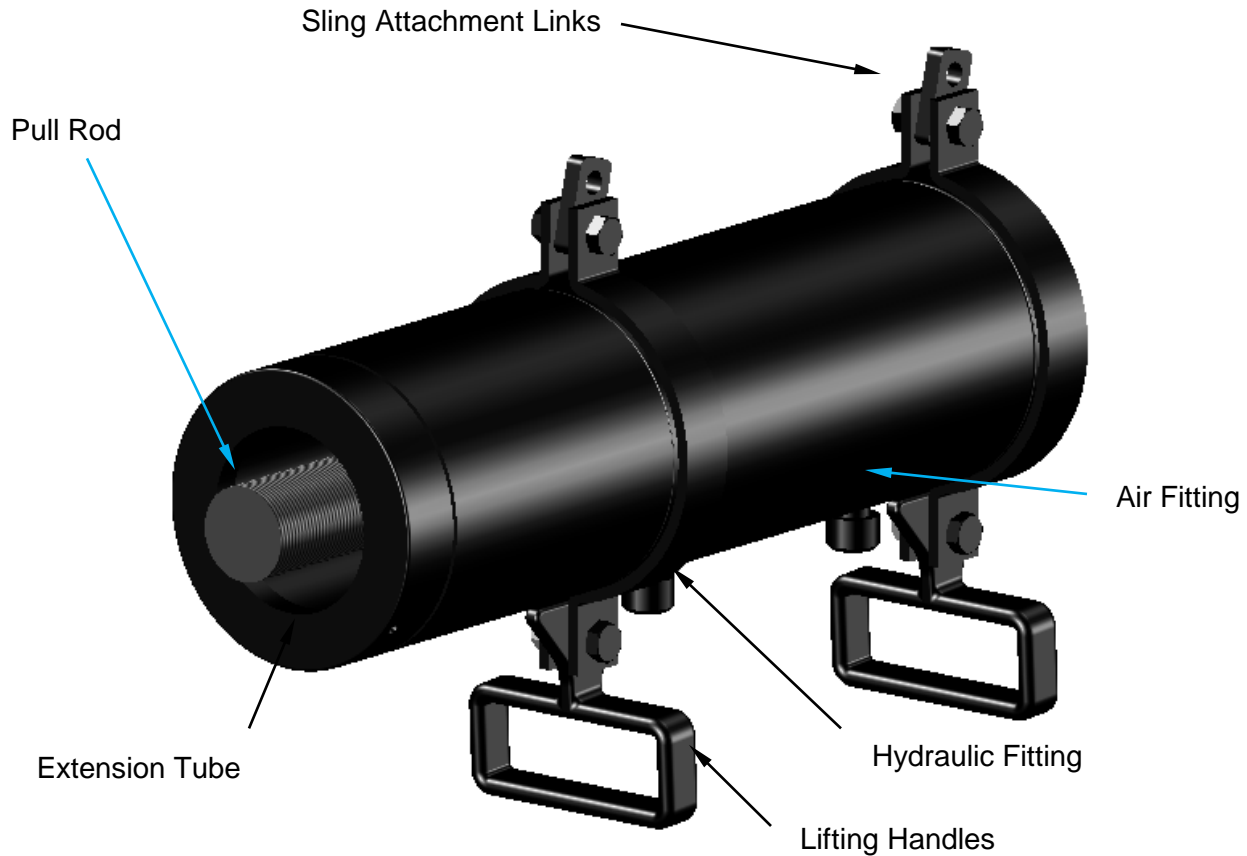
Figure 1.3-1 SB-2A Parts
