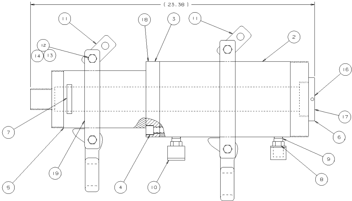
Figure 6.1-1 SB-2A Diagram
