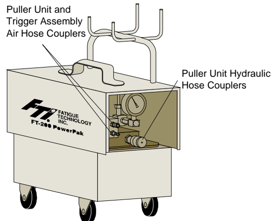
Figure 5.0-1 FT-200 PowerPak
