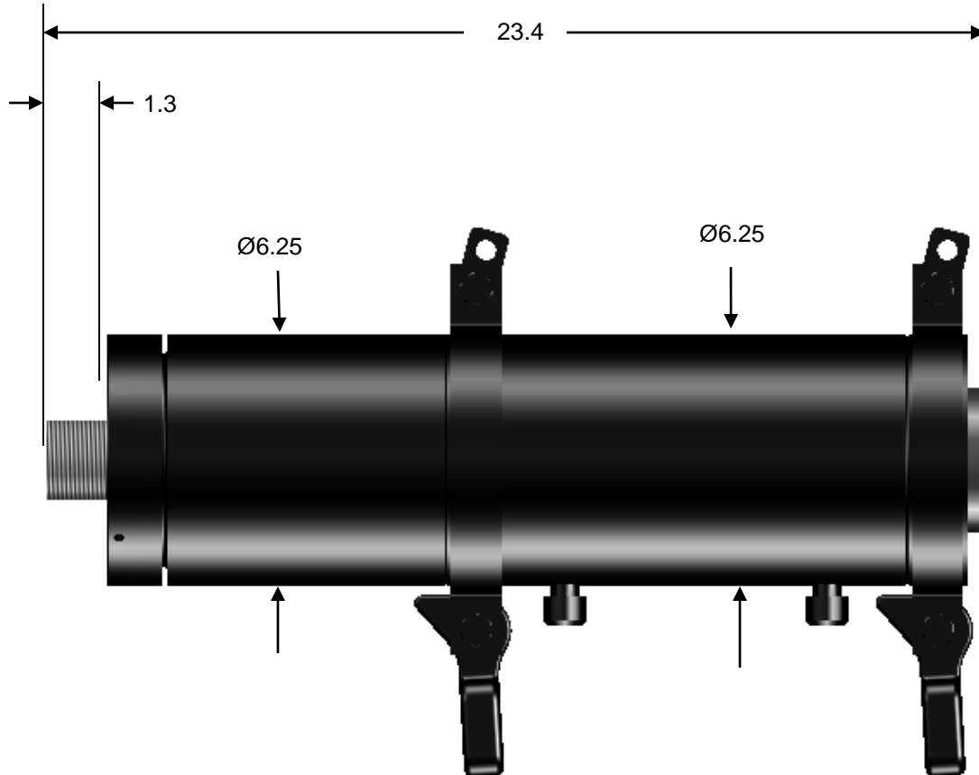
Figure 1.3-2 SB-2A Dimensions
