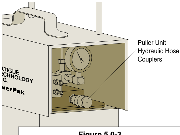
Figure 5.0-3 Location of Hydraulic Quick Coupler
