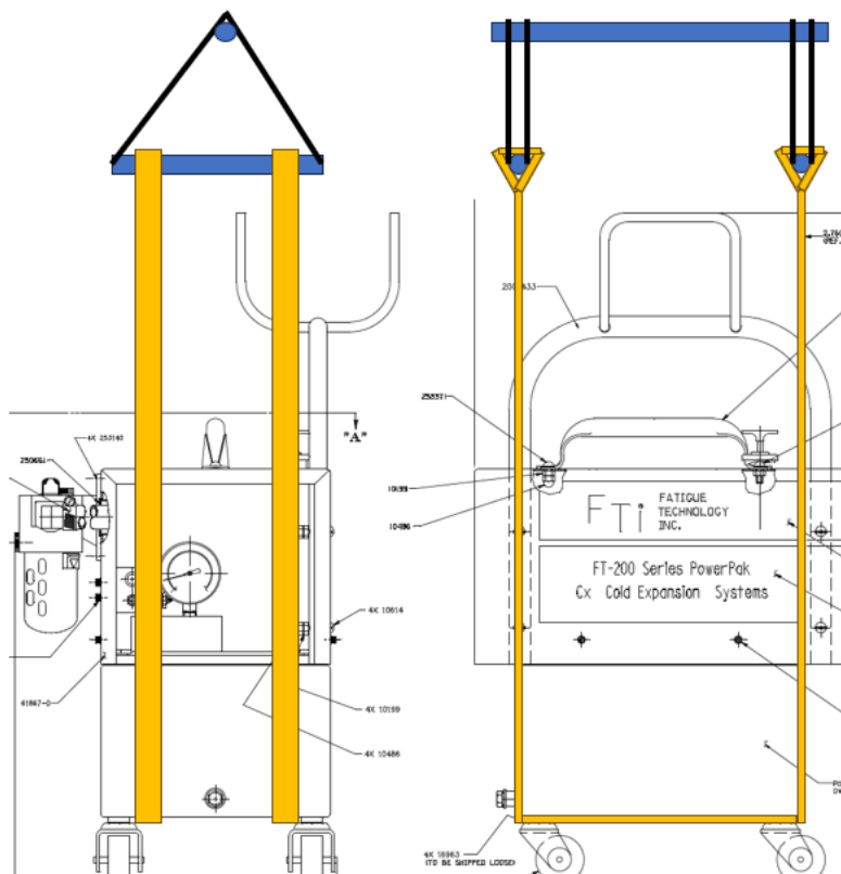
Figure 2.0-5 Example Lifting Method
