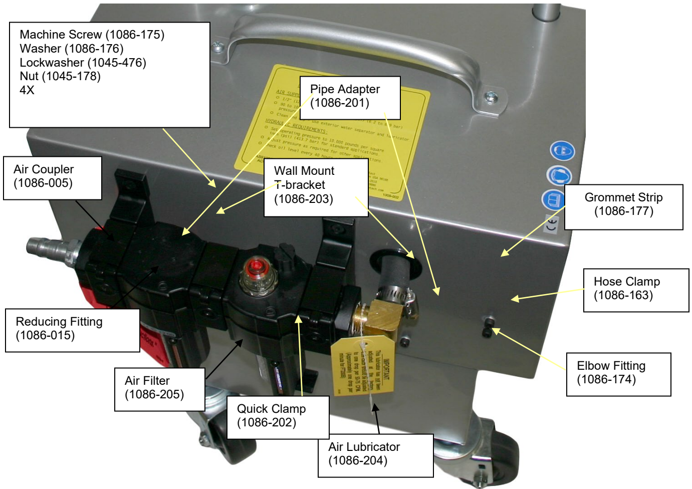
Figure 11.1-2 Conversion Kit
