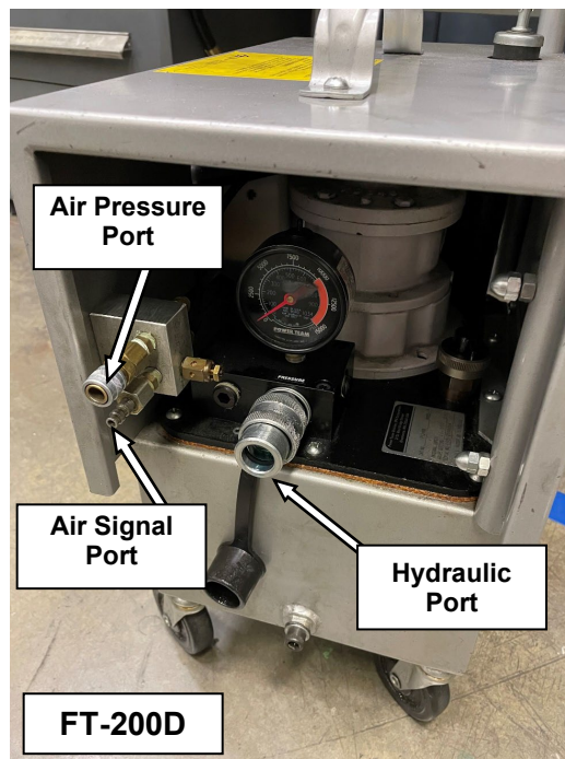
Figure 3.1-1 Port Locations
