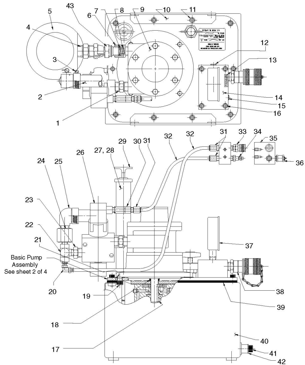
Figure 8.1-1 FT-200M Air Hydraulic Pump
